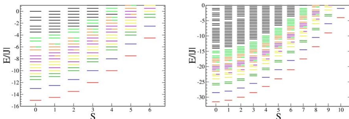
Figure 2. Part of the energy spectra of the rotational-band Hamiltonian for a cuboctahedron with twelve spins s = 1 (left) and s = 3/2 (right). Seven super-bands are colored.
