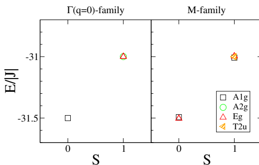
Figure 4. Classification by irreducible representations of O_h of the quasi-classical states with lowest energies of the \Gamma(q=0) -family and M -family within S=0 and S=1 subspaces. The given energies refer to a diagonalization of the Heisenberg Hamiltonian exclusively within these quasi-classical states in the system with s=3/2 .
