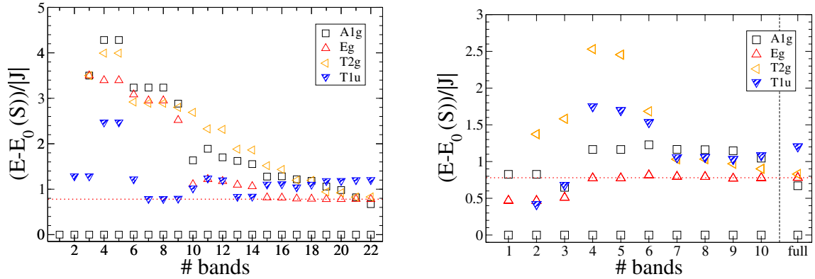
Figure 6. Energy difference to the ground state of selected low-lying energy levels of the cuboctahedron s = 1 within S = 0 subspace depending on the number of incorporated rotational bands. The reduced set of basis states is taken from rotational-band states of the \Gamma(q = 0) -family only (left) and from linear combinations of states of all four colorings (right). The classification is according to O_h point-group symmetry. The dotted red line refers to the exact difference from the E_g -state.
