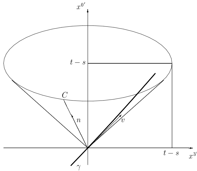
Fig. 2 In the particle's momentarily comoving frame the massless charge is placed at the coordinate origin; its 4-velocity is (1, 0, 0, 1) . The point C \in S(0, t - s) is linked to the coordinate origin by a null ray characterized by the angles (\varphi, \vartheta) . (The null vector n = (1, \cos \varphi \sin \vartheta, \sin \varphi \sin \vartheta, \cos \vartheta) defines this direction.) For a given point C with coordinates x^{\alpha'} = (t - s)n^{\alpha'} the retarded distance is x^0 - x^3 = (t - s)(1 - \cos \vartheta) .
