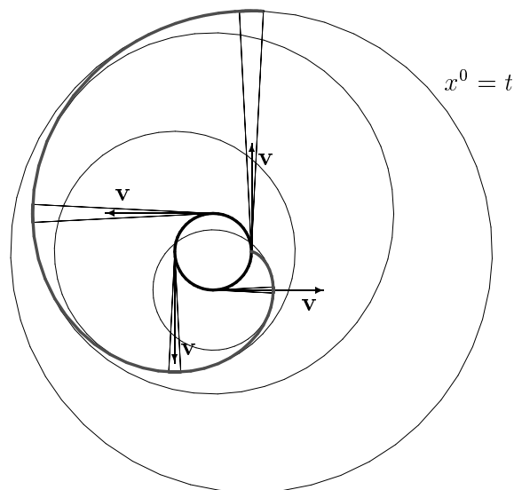
Fig. 3 The bold circle pictures the trajectory of a photon-like charge. The others are spherical wave fronts (21) viewed in the observation hyperplane \Sigma_t = \{x \in \mathbb{M}_4 : x^0 = t\} . The circling photon-like charge radiates infinite rates of energy-momentum and angular momentum in the direction of its velocity \mathbf{v} at the instant of emission. The energy-momentum and angular momentum carried by electromagnetic field of accelerated charge tend to infinity on the spiral curve.
