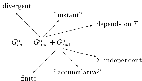
Fig. 1 The bound term G_{bnd}^\alpha and the radiative term G_{rad}^\alpha constitute Noether quantity G_{em}^\alpha carried by electromagnetic field. The former diverges while the latter is finite. Bound component depends on instant characteristics of charged particles while the radiative one is accumulated with time. The form of the bound term heavily depends on choosing of an integration surface \Sigma while the radiative term does not depend on \Sigma .
