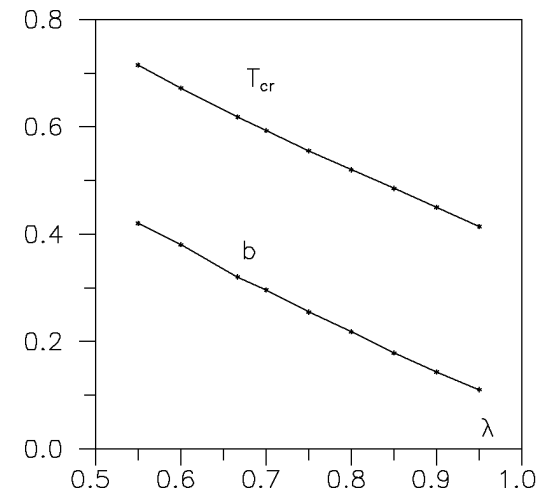
Figure 8. Critical index b defined by m_3(\beta) = A(T_{cr} - T/T_{cr})^b and T_{cr} via \lambda .
