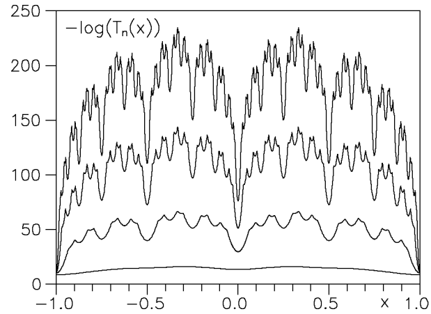
Figure 5. -\log T_n(x) via x = \xi/m_n(\beta) for n = 15, 20, 23, 25 subsequently, the lowest curve is for n = 15 .
