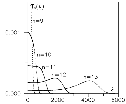
Figure 3. T_n(\xi) via \xi for n = 9, \dots, 13 and \lambda = 2/3, \beta^{-1} = 0.61 .
