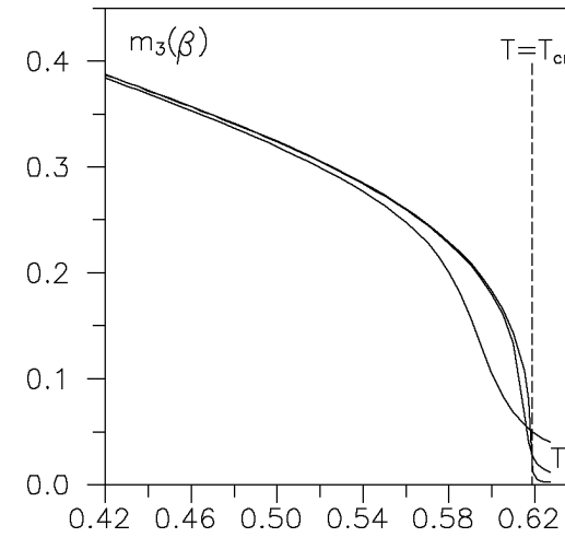
Figure 7. m_3^{(n)}(\beta) given by (3.15) via T = \beta^{-1} for \lambda = 2/3 and n = 10, 15, 20 subsequently, the lowest curve is for n = 10 .
